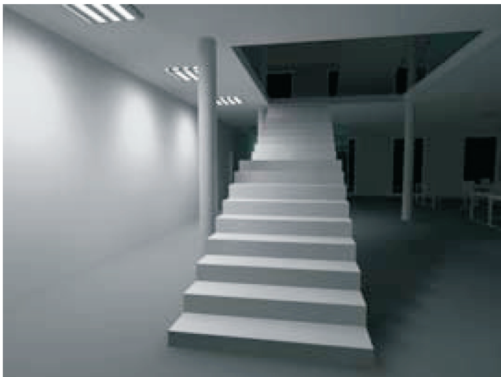
Scale: 1 : 50 Horizontal illuminance (Grid) Average: 226 lx, Min: 148 lx, Max: 268 lx, Min/average: 0.655, Min/max: 0.552, Points: 3 x 9 (Relevant: all)
