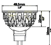
MR16 / 4.5W
