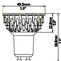
GU10 / 4.5W
